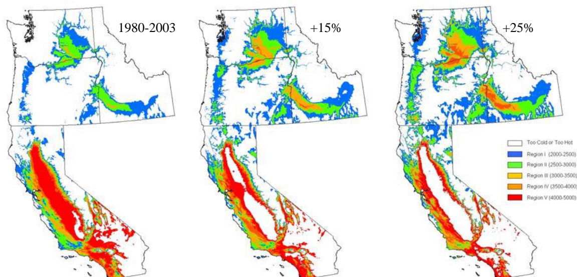
Figure 5 – Winkler Regions for the western U.S. based on Daymet (Thornton et al., 1997) daily 1 km resolution daily temperature data (growing degree-days, base 50°F over Apr-Oct). The left panel is the average over the 1980-2003 time period. The middle panel is a projection of a 15% increase over 1980-2003 (low range of climate change expected by 2049). The right panel is a projection of a 25% increase over 1980-2003 (high range of climate change expected by 2049).
