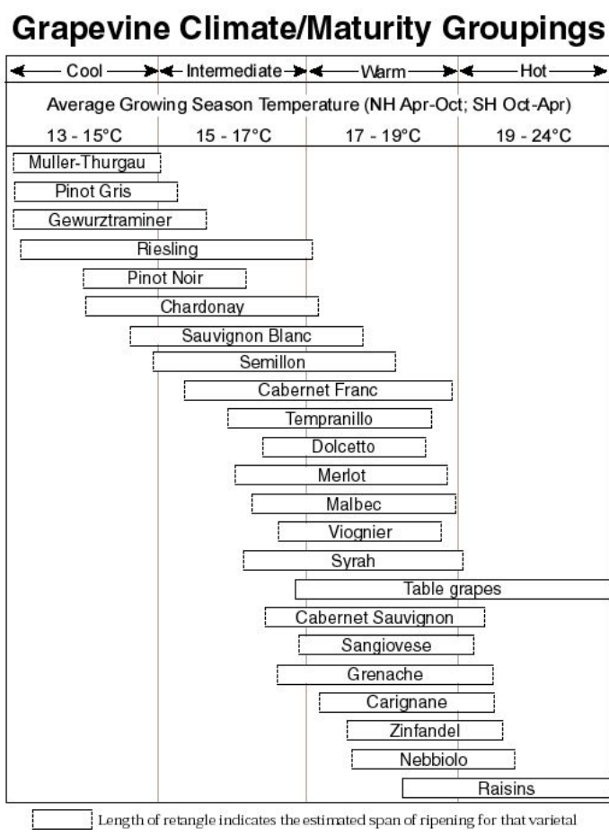
Figure 1 – The climate-maturity groupings given in this figure are based on relationships between phenological requirements and climate for high to premium quality wine production in the world's benchmark regions for each variety. The dashed line at the end of the bars indicates that some adjustments may occur as more data become available, but changes of more than +/- 0.2-0.6°C are highly unlikely. The figure and the research behind it are a work in progress (Jones, 2006).
