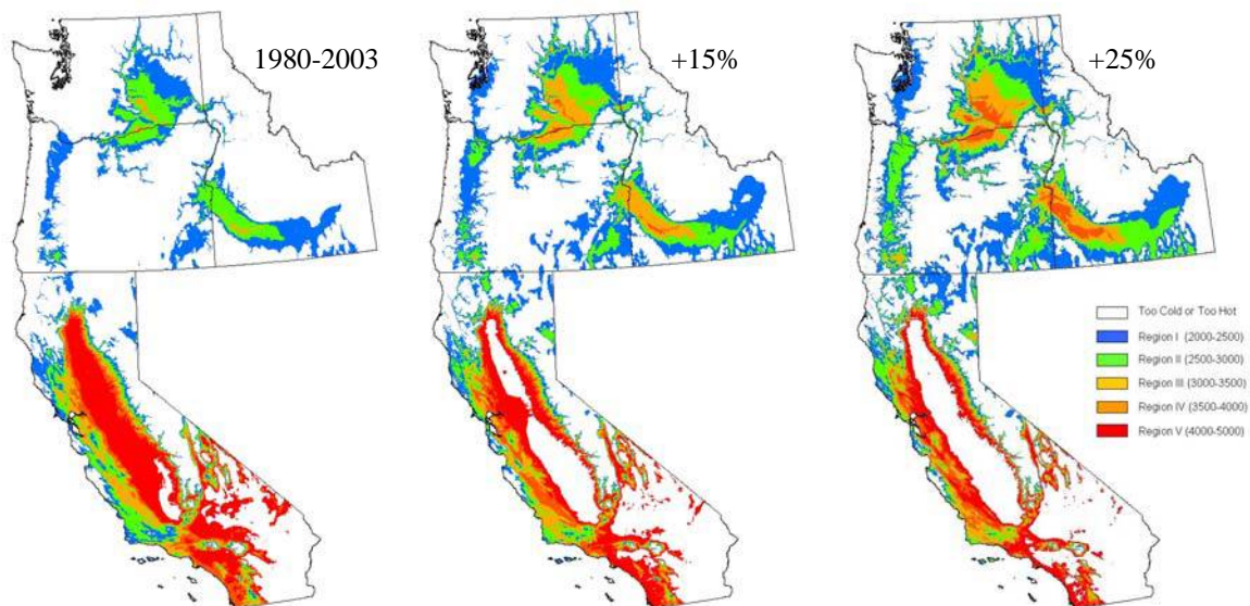
Figure 5 – Winkler Regions for the western U.S. based on Daymet (Thornton et al., 1997) daily 1 km resolution daily temperature data (growing degree-days, base 50°F over Apr-Oct). The left panel is the average over the 1980-2003 time period. The middle panel is a projection of a 15% increase over 1980-2003 (low range of climate change expected by 2049). The right panel is a projection of a 25% increase over 1980-2003 (high range of climate change expected by 2049).
