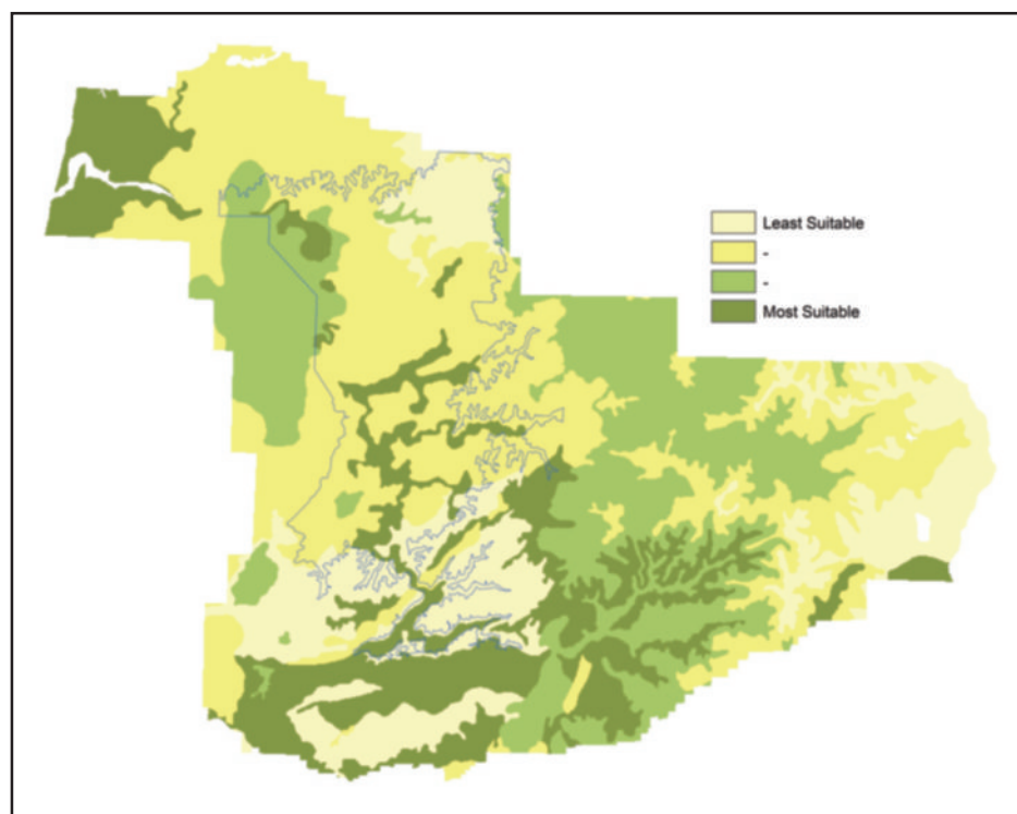
Figure 6 Soil suitability as defined through the combination of drainage, depth to bedrock, available water-holding capacity, and pH. The results are depicted for Douglas County as a whole and with the Umpqua Valley AVA outlined in blue.
