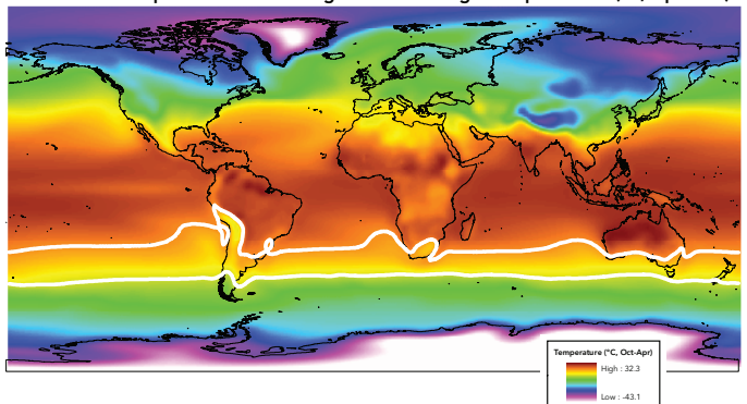
Figure 3. Maps of growing season average temperatures (Northern Hemisphere, Apr–Oct upper panels; Southern Hemisphere, Oct–Apr lower panels) derived from observations and model runs from the Community Climate System Model (CCSM). The left panel is the 1999 run and the right panel is for the 2049 run. Future projections are driven by the A1B emission scenario (moderate future consumption). The highlighted isotherms (white) are the mean 12\text{--}22^{\circ}\text{C} representing the latitudinal limits of the majority of the world's grape growing areas (Gladstones 2005; Jones 2006)
