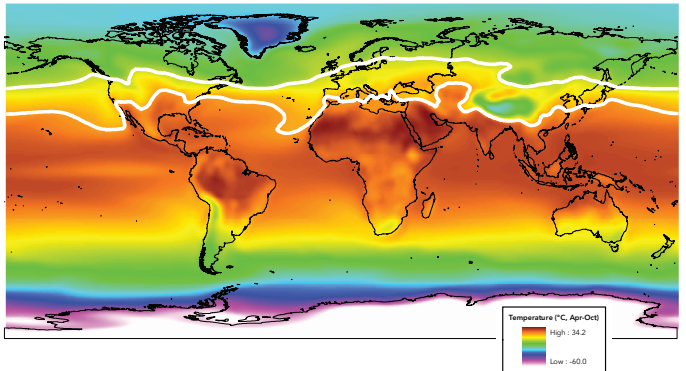
Northern Hemisphere 2049 Growing Season Average Temperatures ( ^{\circ}\text{C} , Apr–Oct)
