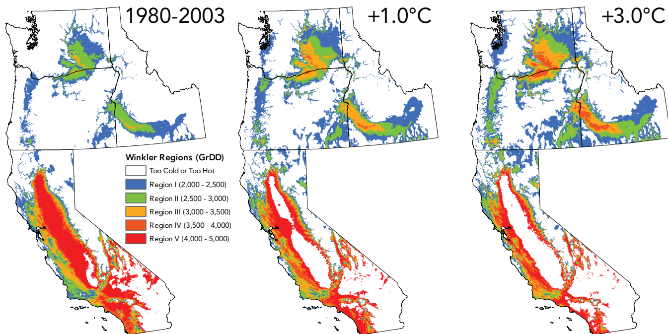
Figure 5. Winkler Regions for the western U.S. based on Daymet (Thornton et al. 1997) daily 1 km resolution daily temperature data (growing degree-days, base 10°C over Apr–Oct). The left panel is the average over the 1980–2003 time period. The middle panel is a projection of a +1.0°C increase over 1980–2003 (low range of projected climate change by 2049). The right panel is a projection of a +3.0°C increase over 1980–2003 (high range of projected climate change by 2049)
