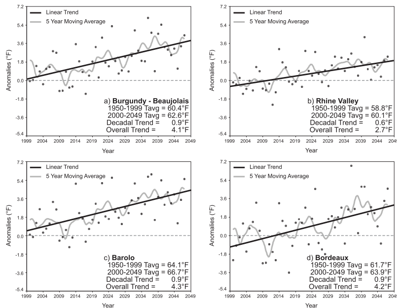
Figure 4. Modeled growing season average temperature anomalies for a) the Beaujolais region of Burgundy, b) the Rhine Valley, c) Barolo, and d) Bordeaux as analyzed by (Jones et al. 2005a). The modeled temperature data are from the HadCM3 climate model on a monthly time scale extracted from a 2.5° x 3.75° grid centered over the wine producing regions for 2000–2049. The anomalies are referenced to the 1950–1999 base period from the HadCM3 model. Trend values are given as an average decadal change and the total change over the 50-year period
