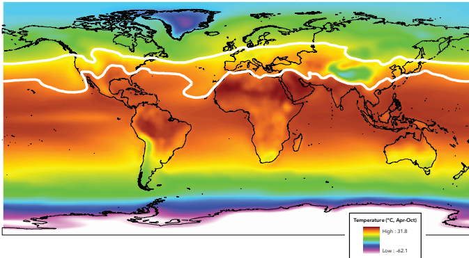
Northern Hemisphere 1999 Growing Season Average Temperatures ( ^{\circ}\text{C} , Apr–Oct)
