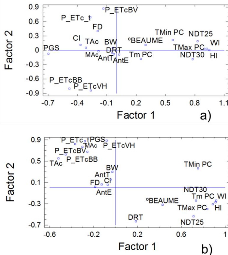
Figure 2. Relationship between climate and grape ripening variables: a) plots on the river terraces; b) plots on the hillslopes.
