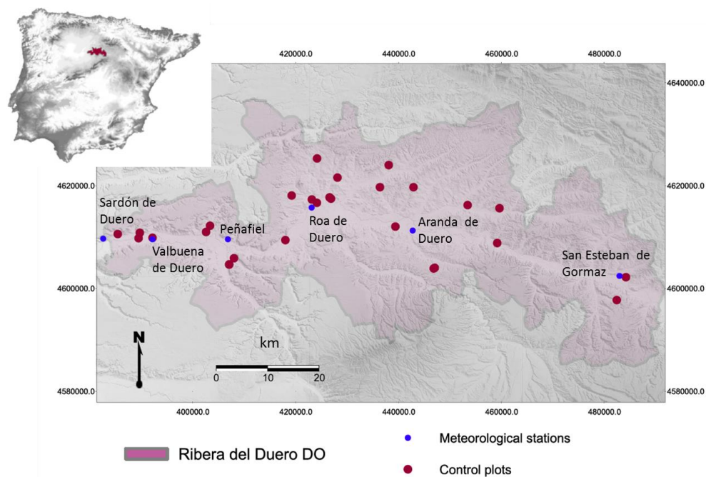
Figure 1: Location of the study area, meteorological stations and plots used in the analysis.
